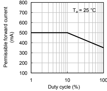
Permissible Forward Current vs. Duty Cycle
