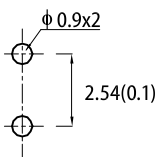
Recommended PCB Layout
