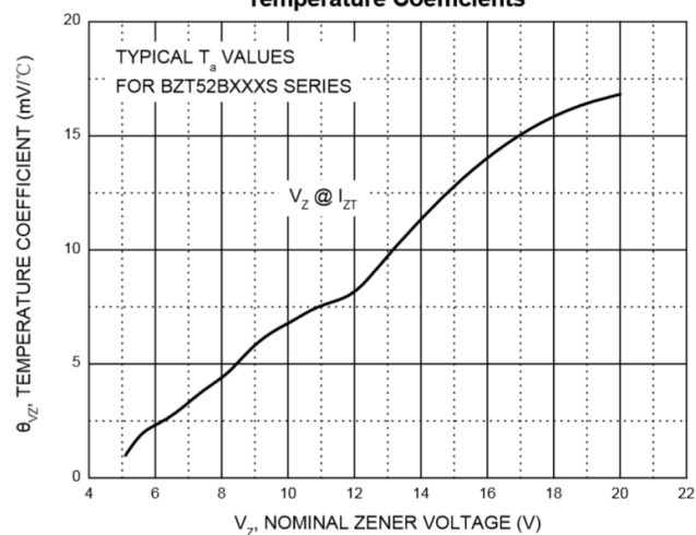
Temperature Coefficients
