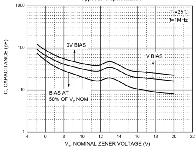
Typical Capacitance
