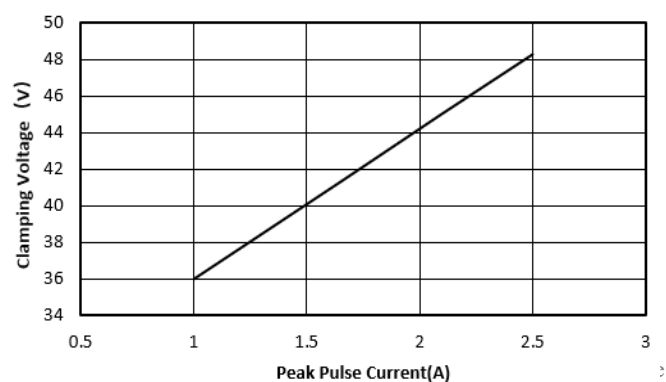
Clamping Voltage VS Peak Pulse Current( t_p=8/20\mu\text{s} )
