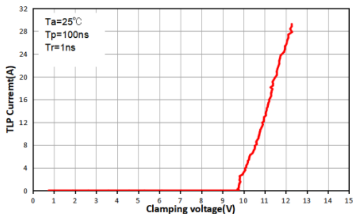
TLP IV curve
