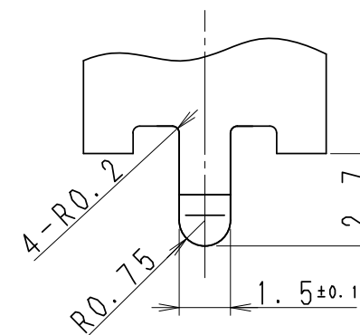
"b" DETAILS (詳細) 5:1
