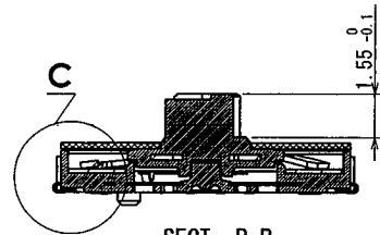
SECT. B-B
