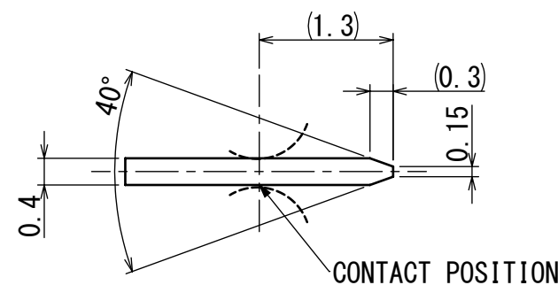
FIG2 INSERTION TERMINAL FORM (VIEW FROM THE DIRECTION OF C)
