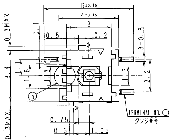
① "DETAIL" 詳細
