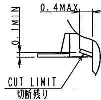
② "DETAIL" 詳細
