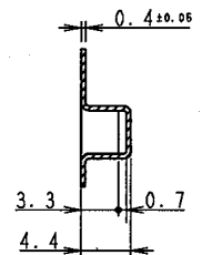
⑤ "DETAIL" 詳細
