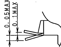
② "DETAIL" 詳細
