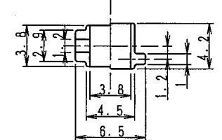
⑤ "DETAIL" 詳細
