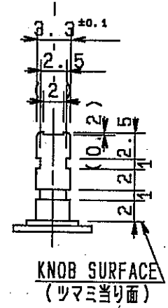
⑧DETAIL(詳細)(2/1)
