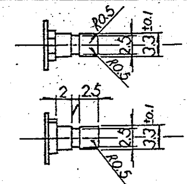
②DETAIL(詳細)( 2/1 )
