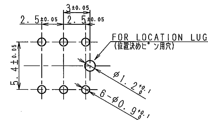
P.C.B. MOUNTING HOLE LAYOUT (基板取付寸法図) (SEE DIRECTION "A") (A方向より見る)
