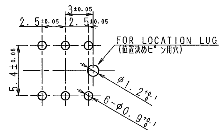
P. C. B. MOUNTING HOLE LAYOUT (基板取付穴寸法図) (SEE DIRECTION "A") (A方向より見る)
