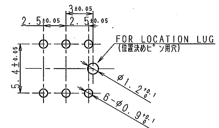
P. C. B. MOUNTING HOLE LAYOUT (基板取付穴寸法図) (SEE DIRECTION "A") (A方向より見る)
