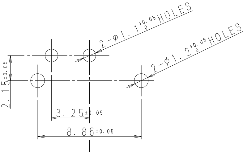
REFERENCE DRAWING FOR MOUNTING HOLES (5:1) 取付穴参考図 (5:1)
