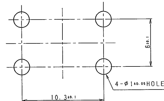
P.C BOARD MOUNTING HOLE DIMENSIONS (WHEN VIEWED FROM SWITCH MOUNTING FACE)
