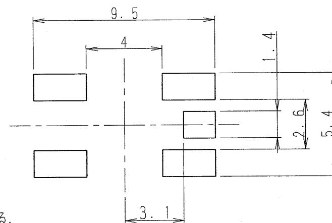
P. C. B推奨パターン図 (5/1) PWB PATTERN DIMENSIONS (5/1)
