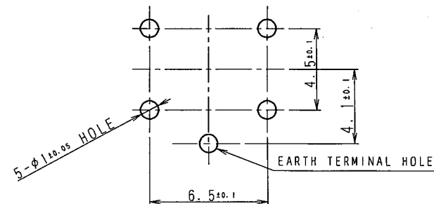
P.C BOARD MOUNTING HOLE DIMENSIONS (WHEN VIEWED FROM SWITCH MOUNTING FACE)
