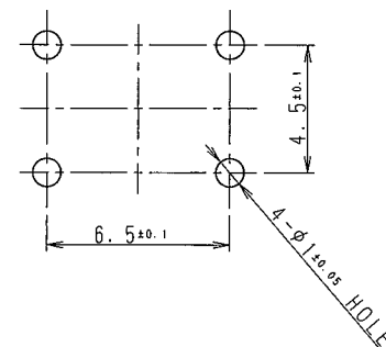
フ° リント基板取付穴寸法図 (スイッチ取付面より見る) PRINTED WIRING BOARD MOUNTING HOLE DIMENSIONS (WHEN VIEWED FROM SWITCH MOUNTING FACE)
