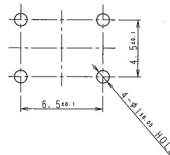
フ リント基板取付寸法図 (スイッチ取付面より見る) PRINTED WIRING BOARD MOUNTING HOLE DIMENSIONS (WHEN VIEWED FROM SWITCH MOUNTING FACE)
