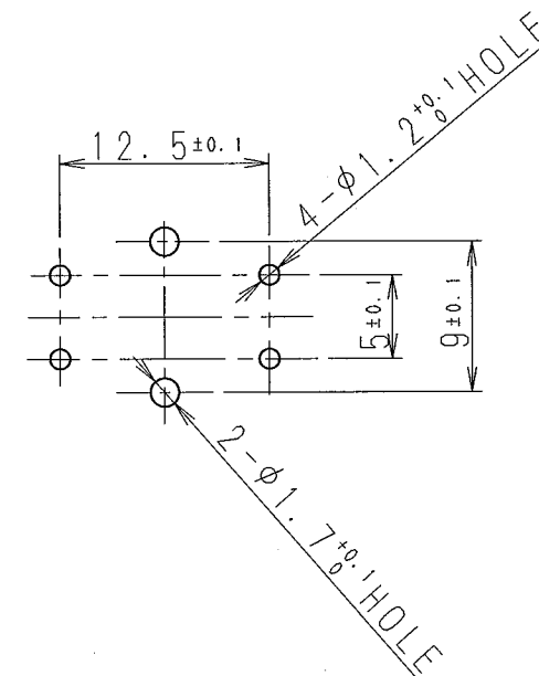
プリント基盤取付穴寸法 (WHEN VIEWED FROM SWITCH MOUNTING FACE)
