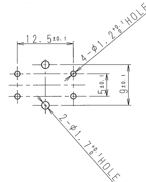
PRINTED CIRCUIT BOARD MOUNTING HOLE DIMENSIONS (WHEN VIEWED FROM SWITCH MOUNTING FACE)
