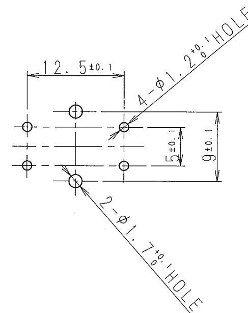
プリント基盤取付穴寸法 (スイッチ取付面側より見る) PRINTED CIRCUIT BOARD MOUNTING HOLE DIMENSIONS (WHEN VIEWED FROM SWITCH MOUNTING FACE)
