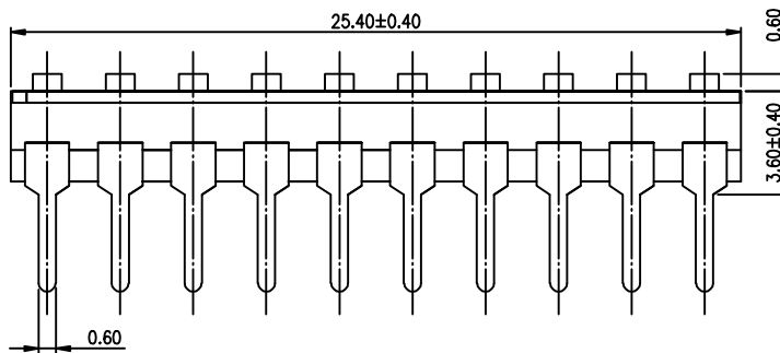
[Schematic]
