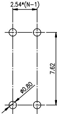
RECOMMENDED P.C.B. LAYOUT (TOP VIEW)
