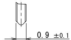
端子先端詳細図 (10:1) DETAIL OF TERMINALS
