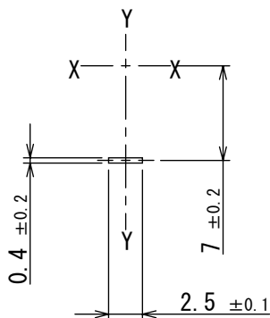
シャシ止め詳細図 LOCATING LUG DETAIL
