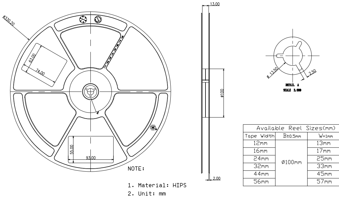
Figure 29. Reel Information
