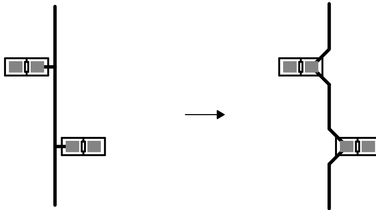
Figure 25. Avoid Stub Traces by Daisy Chain Routing
